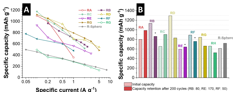
Figure 9. Graphical illustration and overview of the obtained specific capacities after cycling for different iron-based electrodes of the state-of-the-art systems. (A) Comparison of the rate handling performance of different state-of-the-art systems with this work. (B) Comparison of performance stability, comparing the initial capacity and 200 th cycle capacity of different state-of-the-art systems with this work. RA: ref. 45; RB: ref. 43; RC: ref. 46; RD: ref. 44; RE: ref. 47; RF: ref. 48; RG: ref. 49; RH: ref. 50; R-Sphero (this work).
